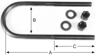
ROUND U-BOLT ASSEMBLY Includes Hi-Nuts and Washers
