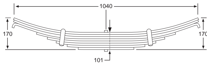
Z-TRA 2172 (8 LEAF)
