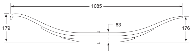
Z-TRA 2291 (3 LEAF)
