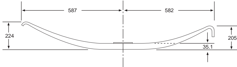
Z-160002 (2 LEAF)
