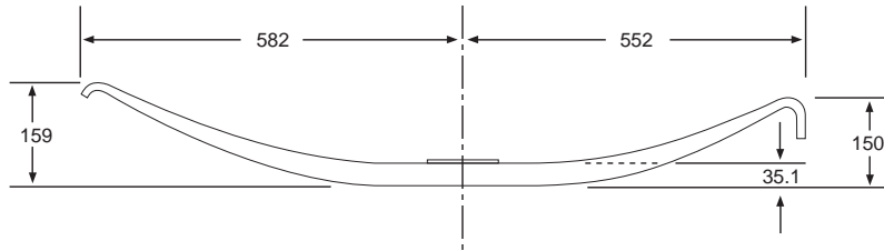
Z-TRA 021 (1 LEAF) low arch
