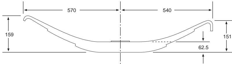
Z-TRA 2728 (3 LEAF) low arch
