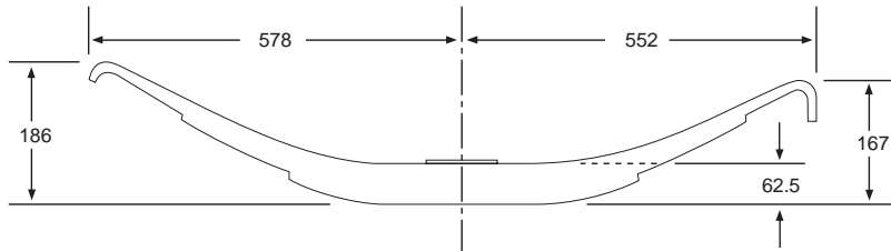
Z-TRA 2727 (3 LEAF) medium arch
