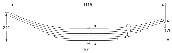
Z-TRA 3310 (8 LEAF)
