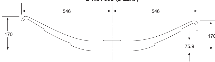
Z-TRA 693 (3 LEAF)
