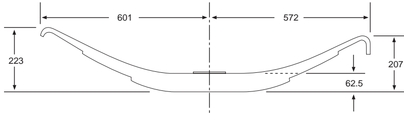
Z-TRA 2726 (3 LEAF) high arch
