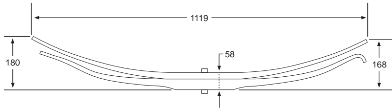
Z-160002 (2 LEAF)
