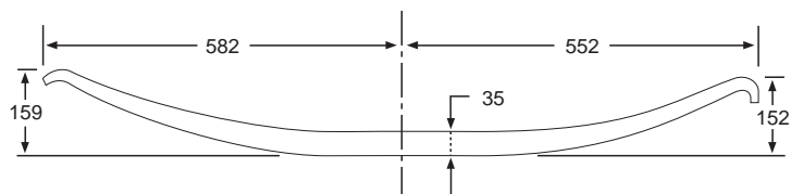
Z-TRA 031 (1 LEAF)
